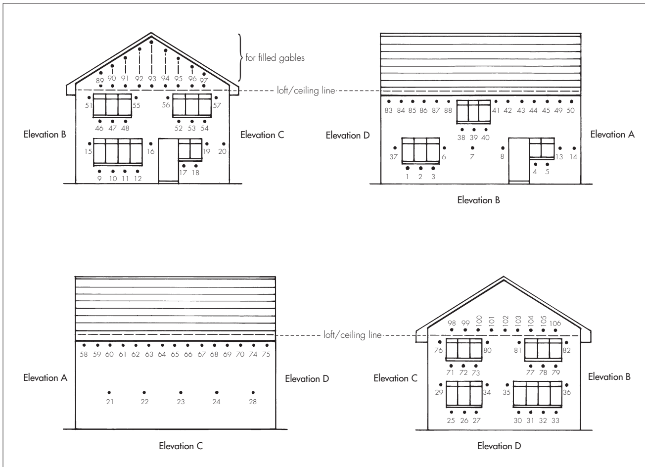
Figure 1 Typical drilling pattern
