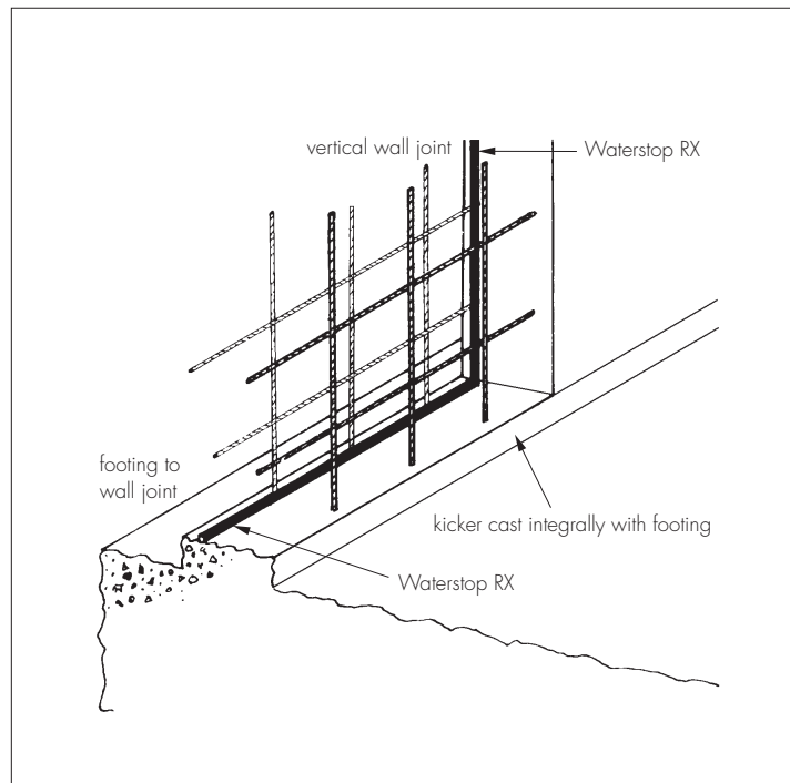
Figure 1 Waterstop RX installation details
