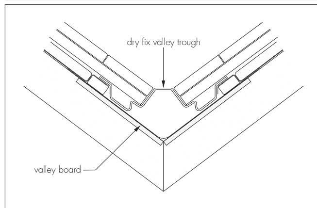
Figure 2 Tile Valley Trough Types DVA and DVB
