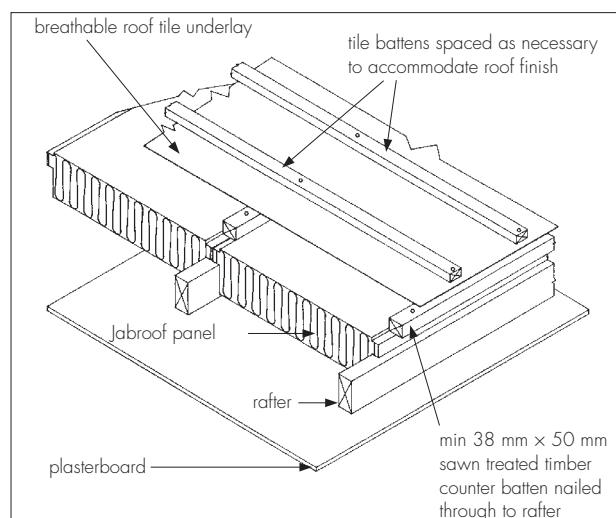
Figure 2 Roof Panel
