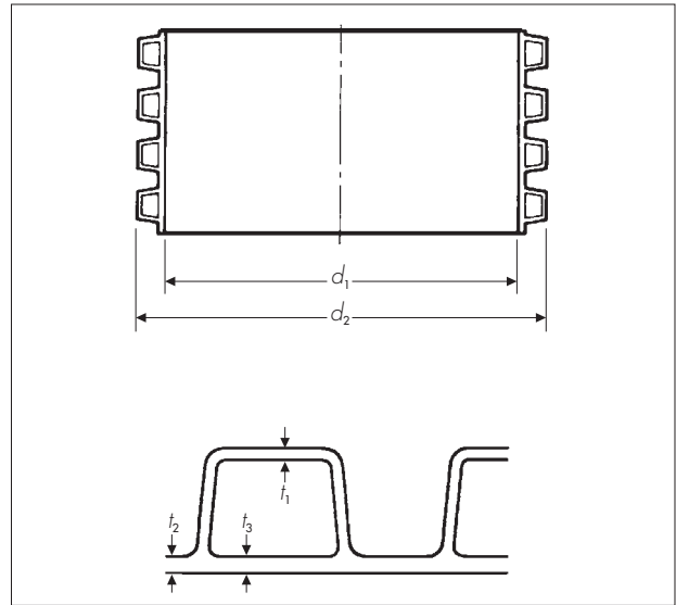
Figure 1 Twinwall pipe
