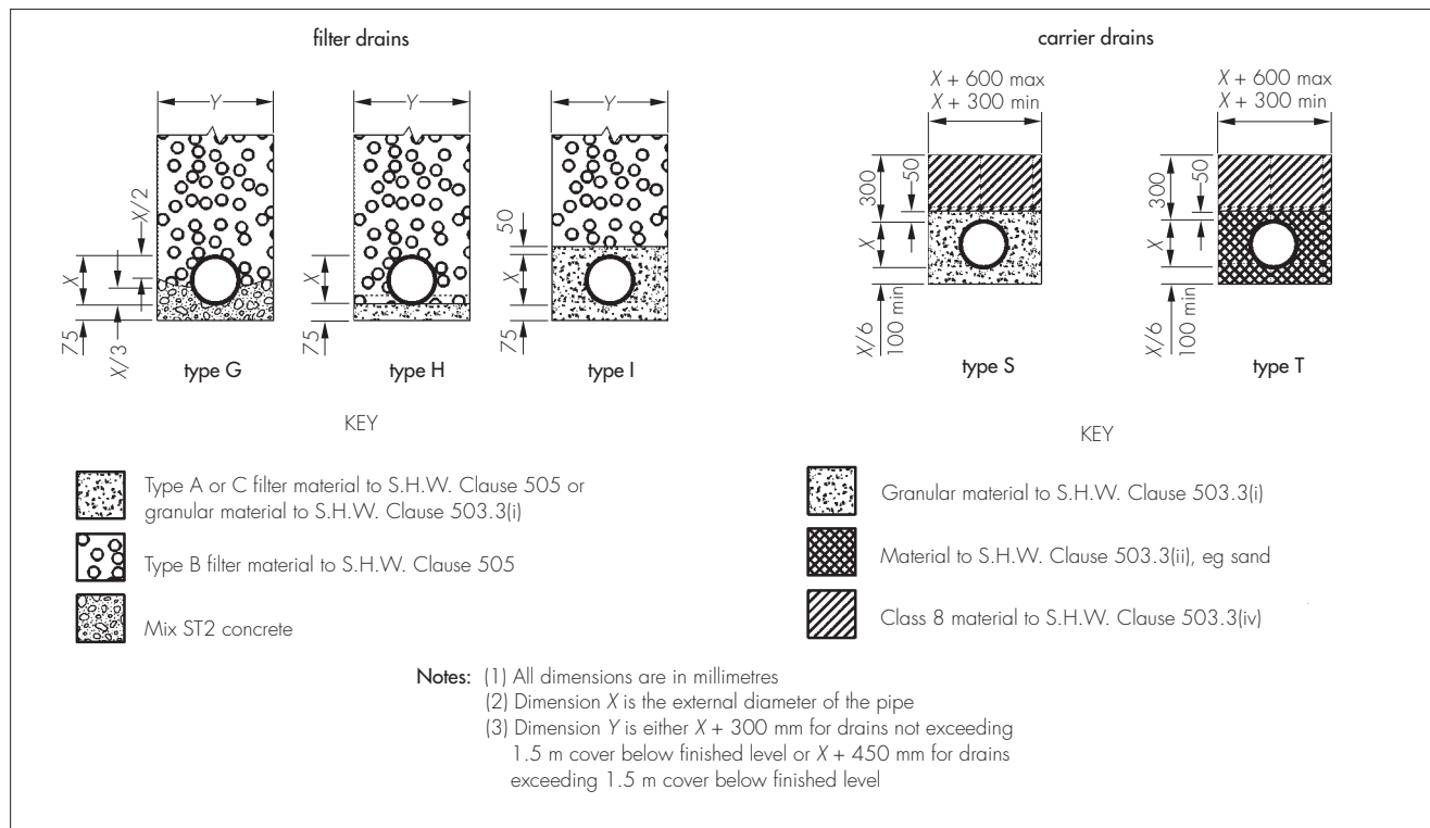
Figure 5 Installation details
