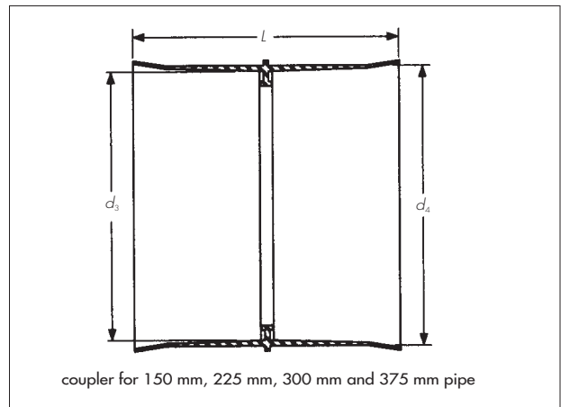
Figure 2 Couplers
