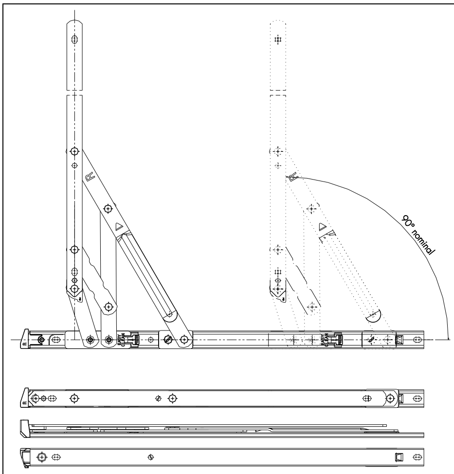
Figure 1 Typical Defender Egress Friction Stays
