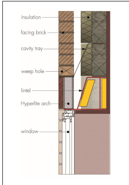
Figure 3 General cross-section of Hyperlite Arch
