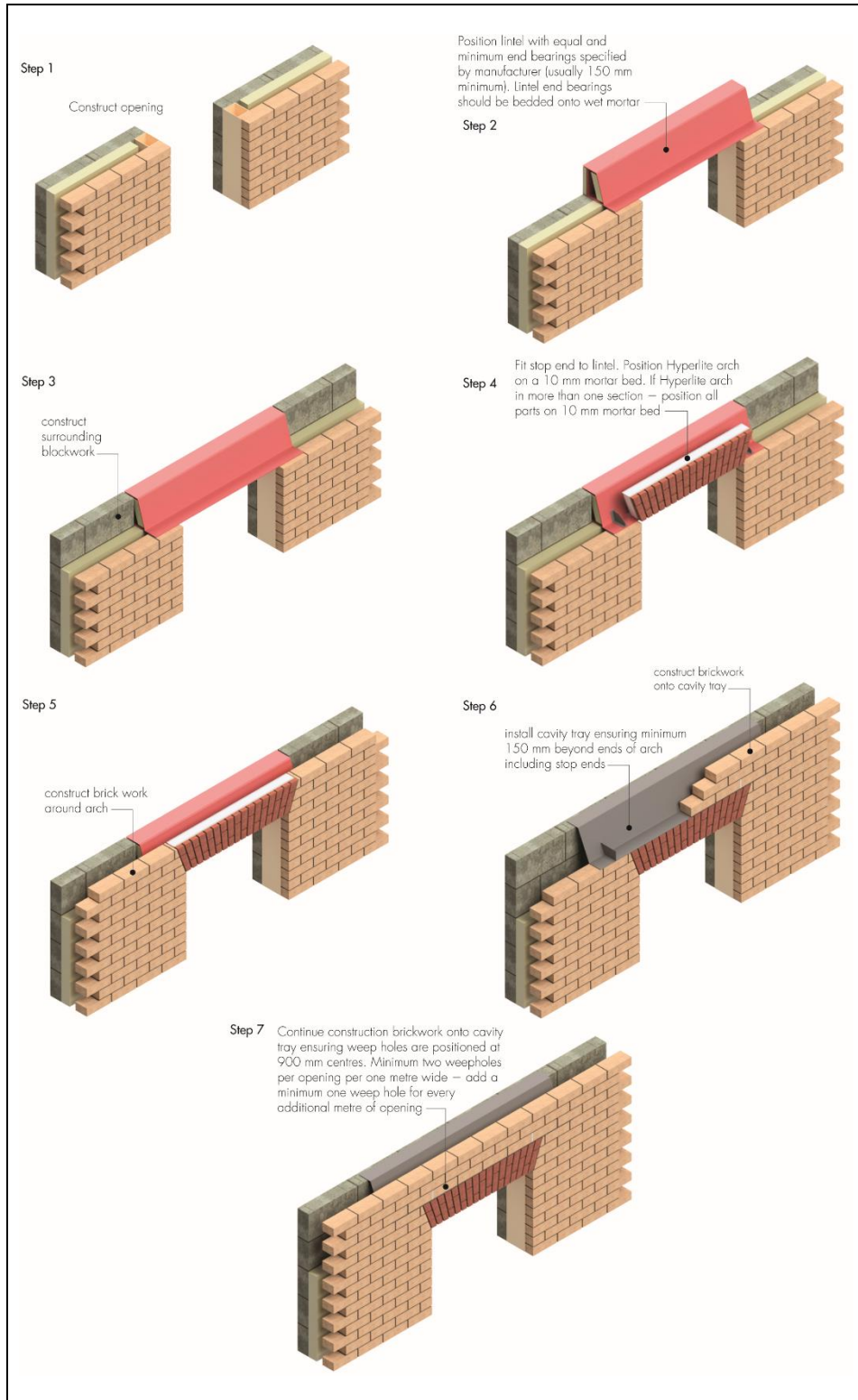
Figure 4 Laying order of Hyperlite Arch
